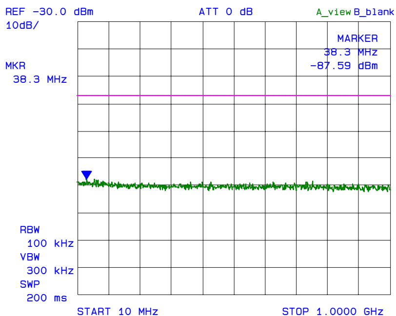
Plot 6.7.5.7 Receiver Conducted Emissions at ANT2 Rx Frequency: 30 MHz
