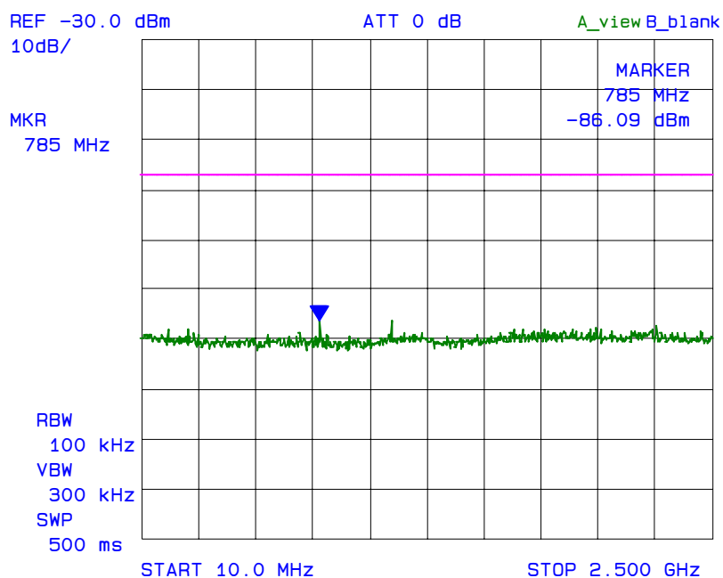
Plot 6.7.5.6 Receiver Conducted Emissions at ANT1 Rx Frequency: 470 MHz
