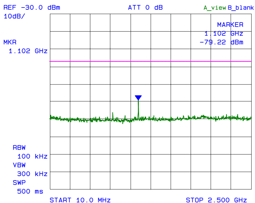
Plot 6.7.5.5 Receiver Conducted Emissions at ANT1 Rx Frequency: 435 MHz
