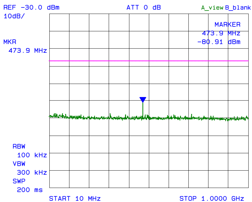
Plot 6.7.5.8 Receiver Conducted Emissions at ANT2 Rx Frequency: 115 MHz
